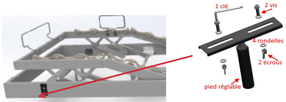
Pied de raccord
